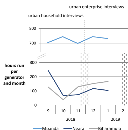
Figure 12: Generator use during survey period
